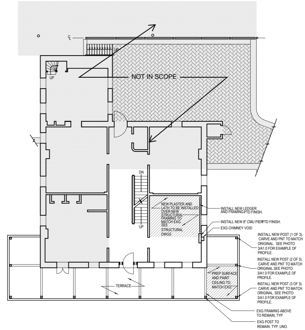
NEW CONSTRUCTION PLAN
