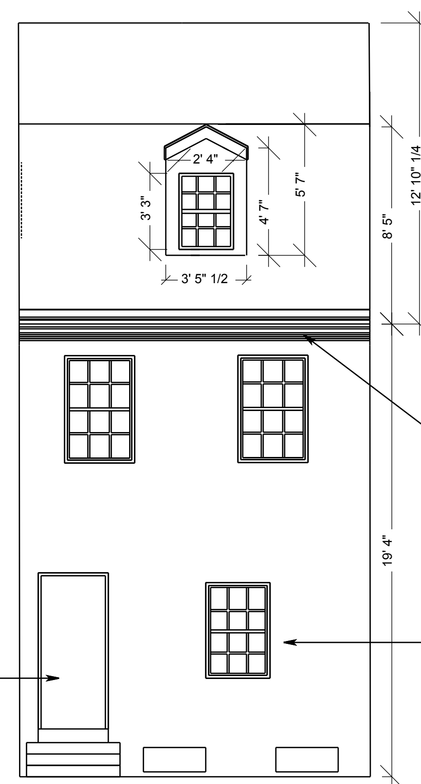
FRONT VIEW
