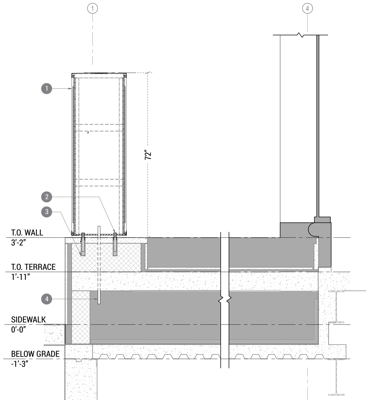
B MONUMENT SECTION SCALE: 1/2"=1'-0"
