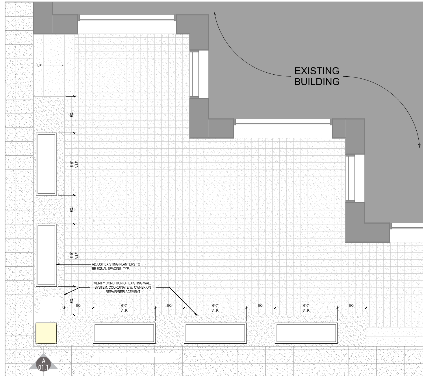
A ENLARGED PLAN SCALE: 3/16"=1'-0"
