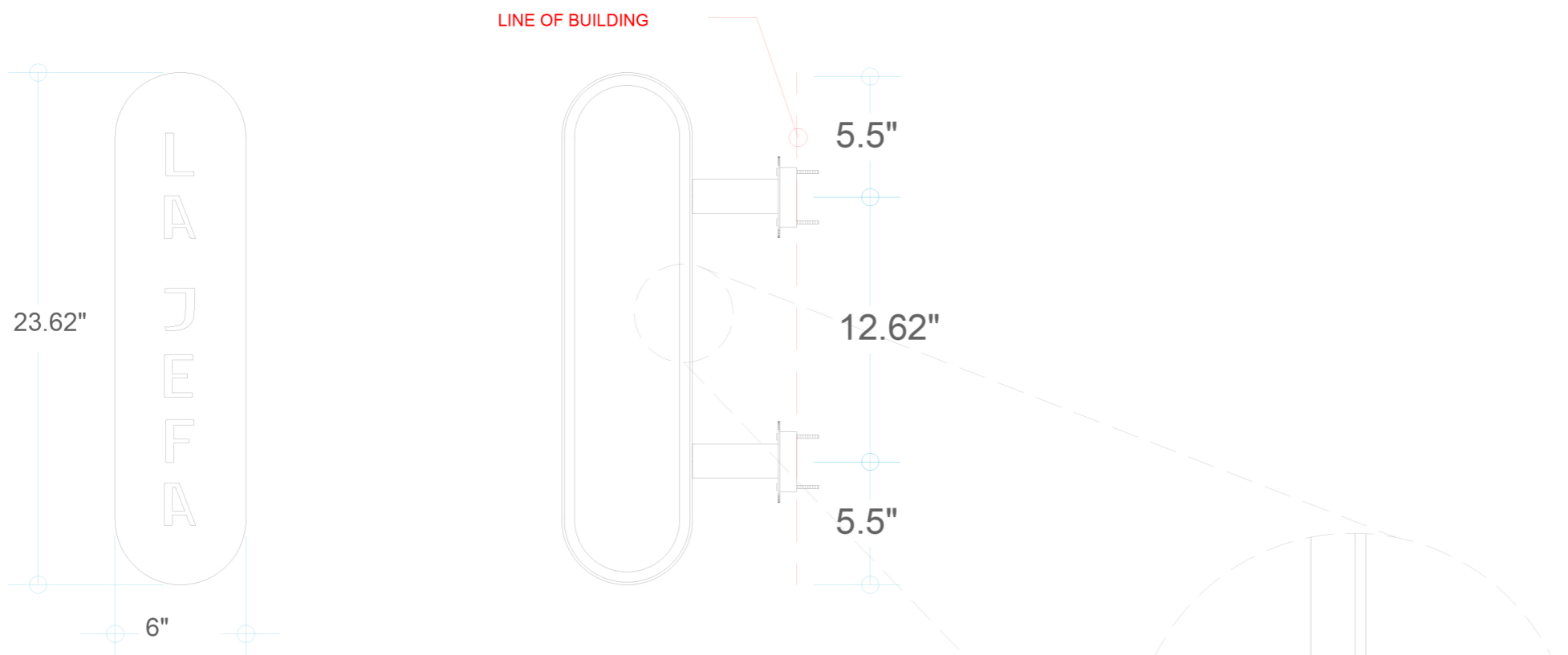
SIGN DETAIL - FRONT
