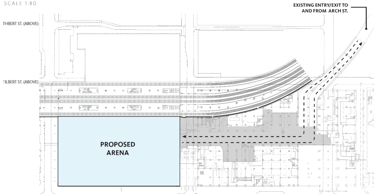
Proposed | Existing Site Loading (2 Levels Below St.). Image source: November 2023 CDR submission
