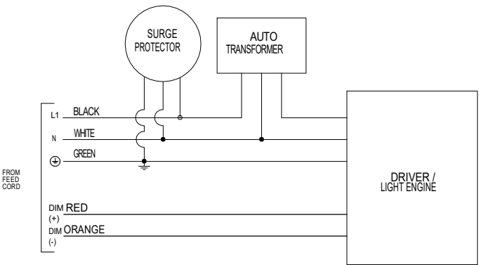
0-10 V Dimming Option (DM) Wiring for 347/480V 100% light output at 10V, down to 1% light output at 0V.
