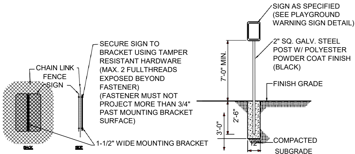
12" X 18" PLAYGROUND WARNING SIGN DETAIL
