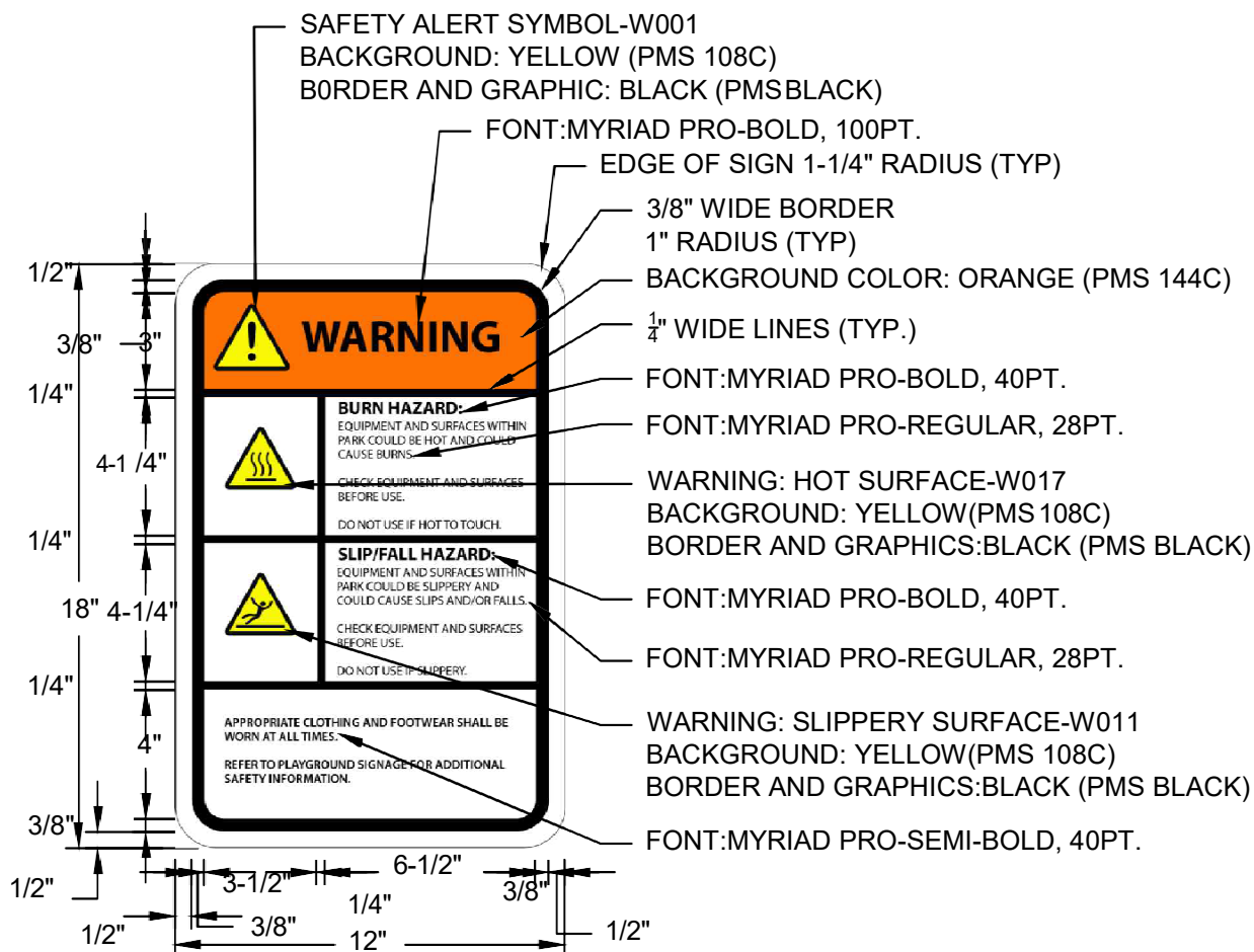
12" X 18" PLAYGROUND WARNING SIGN DETAIL
