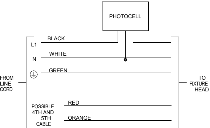
Photocell Wiring Available for all configurations except Short Arm Wall Mount (SW), Single Pole Adapter (SA)
