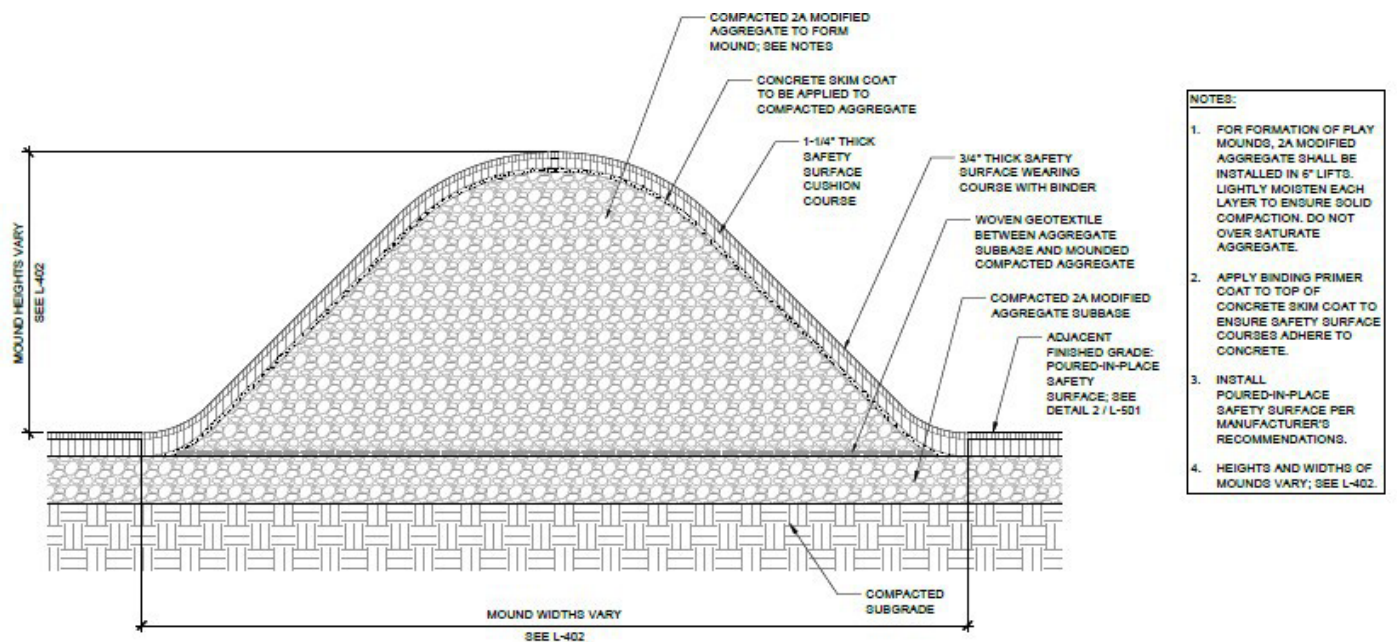
6 PLAY MOUND - TYPICAL
