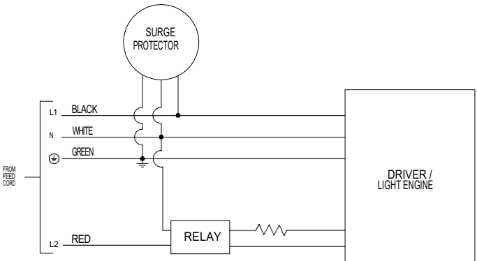
Hi-Lo Switching Option (HLXX) Wiring 120/240/277V. When red is energized, light output will be at "Lo" level.
