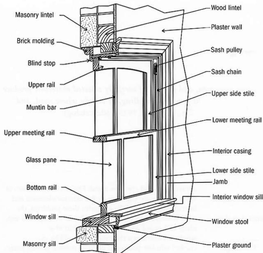
Cross-section of typical double-hung window; view from interior. Illustration: Seaquay Architectural Millwork Corporation.
