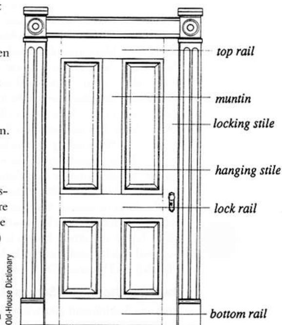
How a door is constructed.
