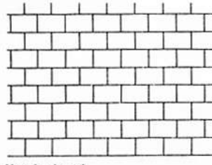
Header bond
